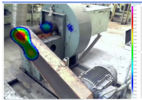
Fig. 5: Visualization of the noise emission intensity of fan driving
