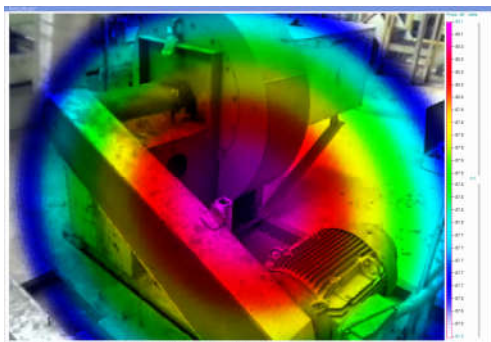
Fig. 6: Visualization of the noise emission intensity of fan driving
