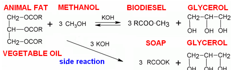
Fig.1: The main reactions of glycerol production
