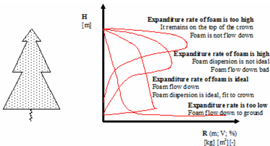
Figure 1 – Structure of foam remaining on the crown depending on the rate of expenditure
